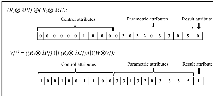
Figure 10. Samples of performing the merge operator ( \oplus ).
