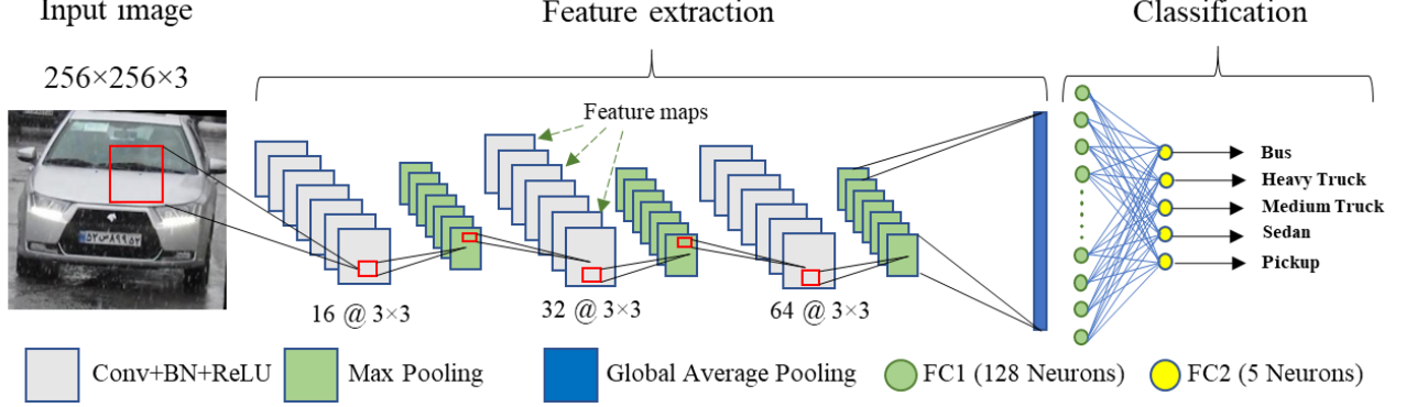
Figure 5. A light weight 3-Conv structure using BN and GAP layers proposed for vehicle classification.
