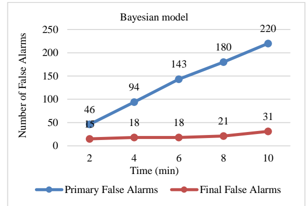
Figure 8. Number of generated false alarms by IDS for three classification models before and after checking the suspicious alarms.
