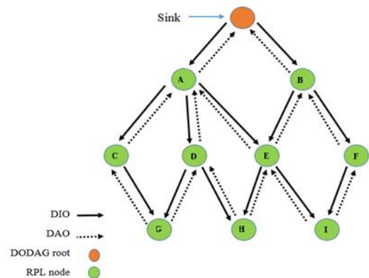
Figure 2. An RPL network control messages DIO and DAO.
