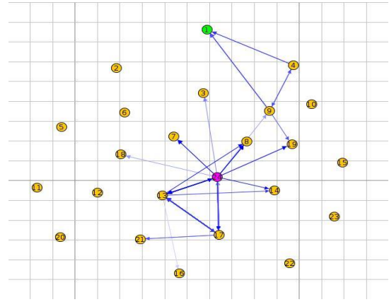
(b) network under sinkhole attack (node 24).
