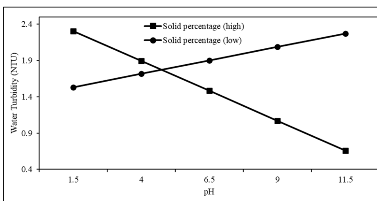
Figure 9. Effect of pulp pH on water turbidity at high and low levels of solid weight percentage (central range of other parameters).
