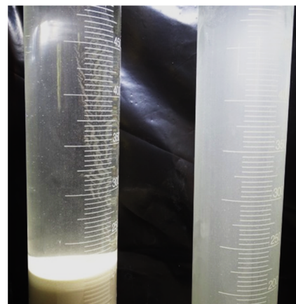
Figure 7. The effect of solid percentage values on water turbidity, Low solid percentage (right), High solids percentage (left).
