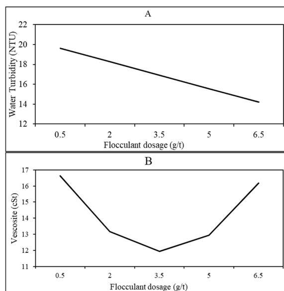
Figure 4. (A) Effect of Flocculant dosage on water turbidity (B) Effect of Flocculant dosage on pulp viscosity, (other factors in the central range).
