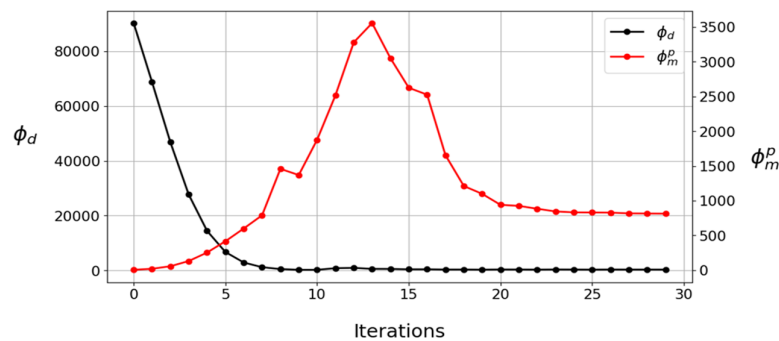
Figure 10. (a) Convergence curve for the case study Inversion. This plot depicts the progress of the susceptibility inversion for the Shavaz deposit. The x-axis represents the number of iterations completed during the inversion. The left y-axis shows the data mis-fit ( \phi_d ), and its decrease after each iteration, indicating a better fit between the model and the observed data. The right y-axis represents the model norm ( \phi_m^p ) and its variations, reflecting the complexity of the estimated subsurface model.
