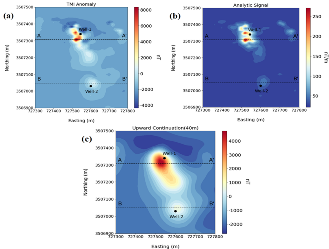
Figure 6. (a) Total Magnetic Intensity (TMI) map following corrections for diurnal variations, International Geomagnetic Reference Field (IGRF), and reduction to the pole, (b) Analytic signal map, (c) Upward continuation map (40 m). The locations of the drilling wells are also indicated.
